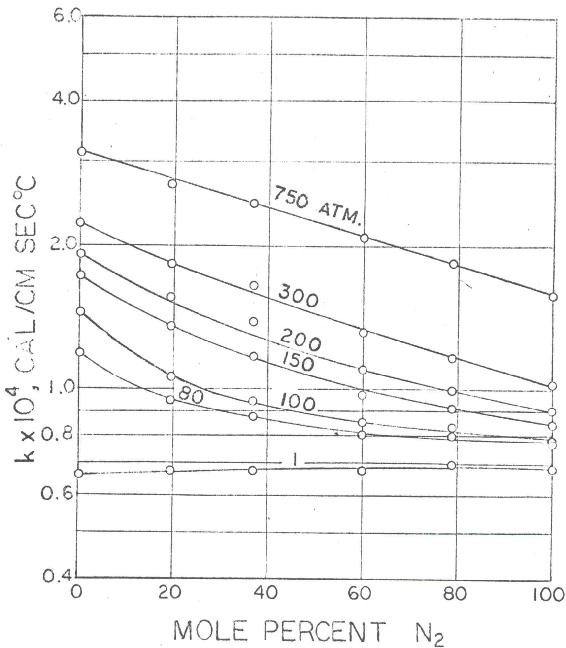
FIGURE 5. THERMAL CONDUCTIVITY OF N 2 -C 2 H 6 MIXTURES AT 75°C
